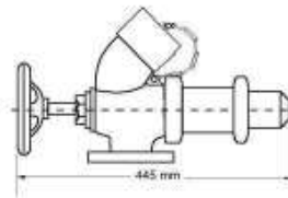
FLANGED SELF REGULATING VALVE
