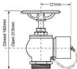
SCREW RIGHT ANGLE VALVE
