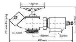
SCREW STANLEY PRESSURE REDUCING VALVE
